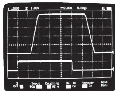
Pulse Response @ R_{TH} = 100 Ohms
