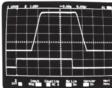
Pulse Response @ R_{TH} = 20 KOhms
