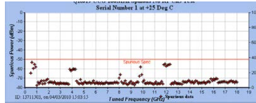
Internally Generated Spurs
