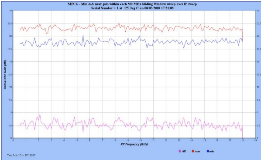
Conversion Gain and GaN Variation
