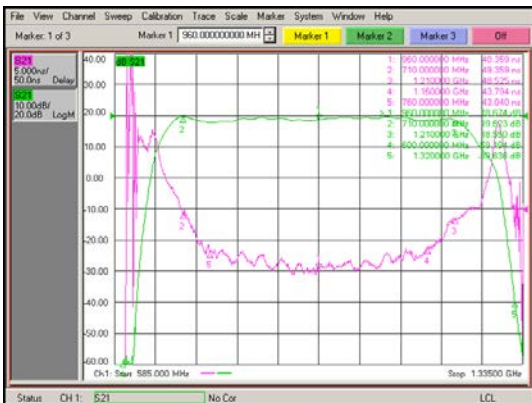
Group Delay and IF Filter Response – Wide IF Bandwidth
