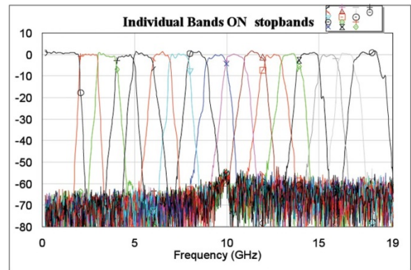
Fig 4. S21, Overlay of individual channels
